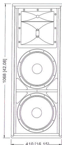
Ktwo-212P Full Range
